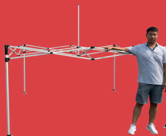
Folding Tent Hex40mm Series
